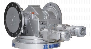
Sun-kissed Robust geared motors for two axes ensure the heliostats keep facing the sun.
